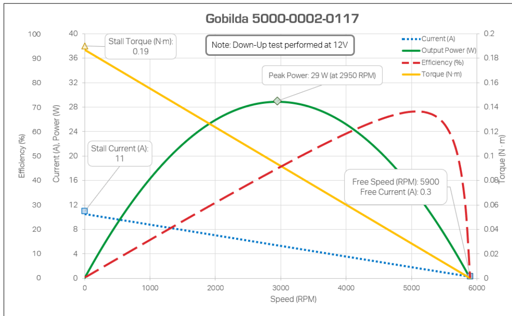
Figure 2: A motor curve graph for one of the motors we plan on using. The yellow line represents the motor torque vs. speed. Source: Game Manual 0. ( https://gm0.org/ro/latest/docs/power-and-electronics/motor-guide/motor-power.html )
